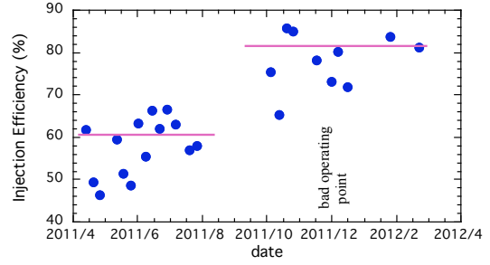
Figure 5: The improvement of the injection efficiency with typical undulator gap in FY2011.
