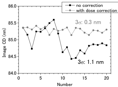
Fig. 6 CD value fluctuation measured by CSM 20 times at the same position of an 88 nm L/S pattern, which shows repeatability of CSM. The two data series show measurements with and without dose correction.
