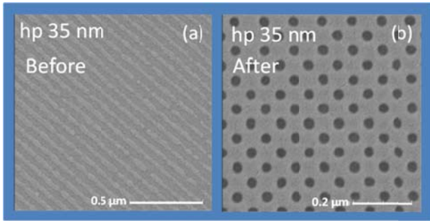
Fig. 9 CD-SEM image of 35-nm-width hole resist (ZEP520A) pattern (a) before and (b) after the vibration improvement.
