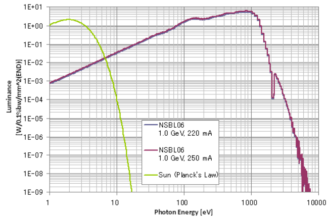
Fig.2 Luminance of BL06 and the sun
