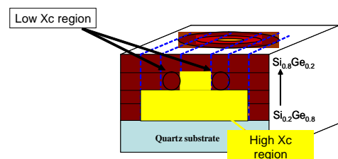
Fig. 2 Cross sectional diagram for crystallization area of SiGe graded film by soft X-ray irradiation.
