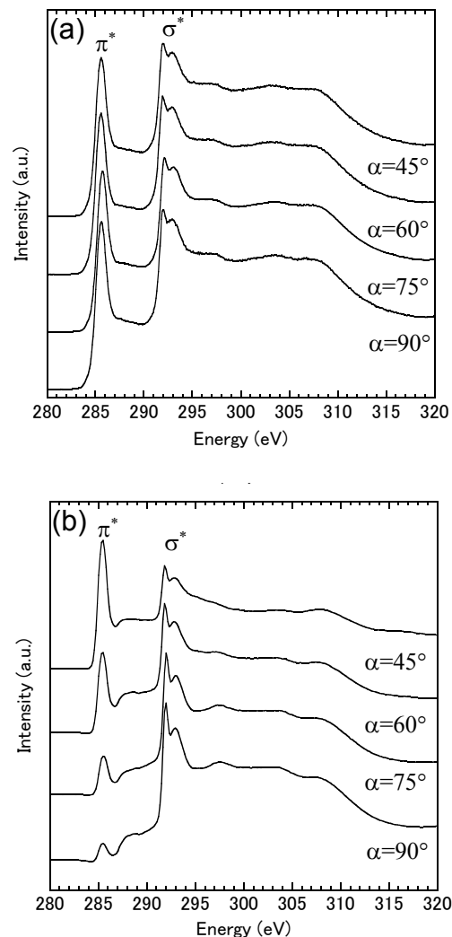
Fig.2. XAS spectra of (a) vertically aligned MWCNT films and (b) multi-layer graphene films at different angles of incident soft x-ray.
