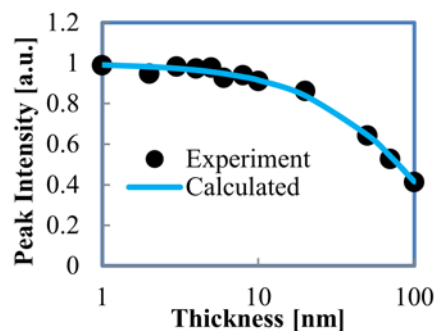
Fig. 3 Thickness dependence of peak intensity at 405 eV of N-K edge of \text{Si}_3\text{N}_4 covered with Cr film measured with the TFY method (circle) and calculated with transmittance of Cr film (line).
