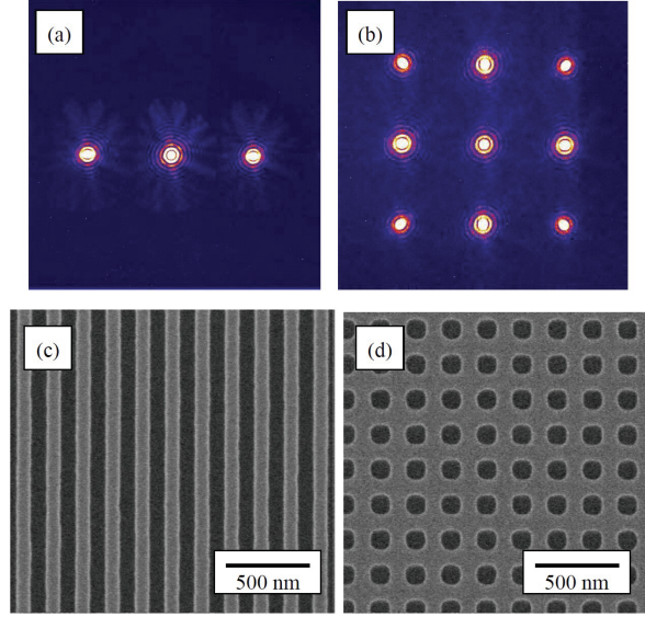
Fig. 3 Diffraction images from the CSM of (a) a 176-nm L/S pattern, and (b) a 112-nm half pitch hole pattern. (c) and (d) are same patterns measured by SEM.
