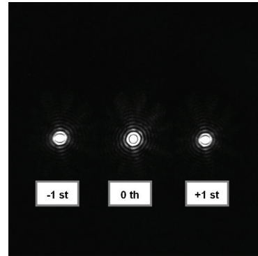
Fig. 3 Diffraction pattern image recorded with the CCD camera from an L/S pattern with 176 nm pitch.
