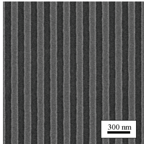
Fig. 5 CD-SEM image of an 88 nm L/S pattern.
