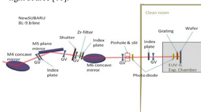
Fig. 1 View of interference lithography system
