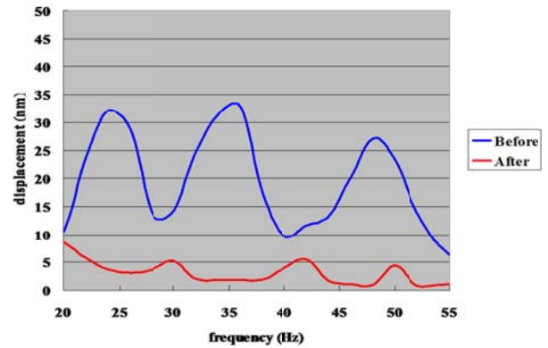
Fig. 6 Vibration of exposure stage
