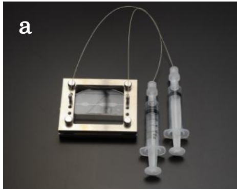
Fig.3: (a) Photo image of microfluidic device. (b) Cross section of microchannel in the microfluidic device (a). Au3D width is 6 mm, height is about 3 \mu\text{m} . Slide glass thickness is 1 mm. PDMS thickness is about 2 mm.
