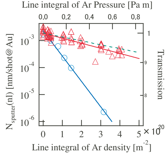
Figure 1 Mitigation of Au sputtering by fast xenon debris (○) and transmission of 13.5 nm soft x-rays (△; experimental, dotted line; Henke et al [4]) as a function of the line integral of the argon pressure.
