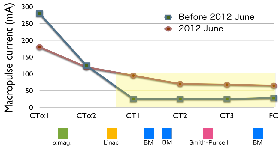
Fig.1 Macropulse current measured by several Current Transformers. Beam transport efficiency was improved after the system upgrades and the fine-tuning.
