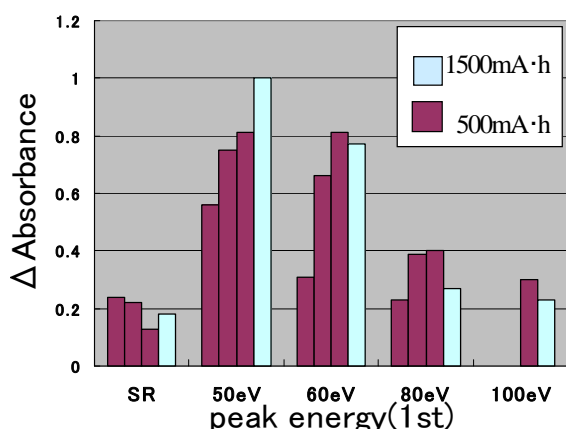
Fig.2 The amount of defects appeared in the absorbance spectra for four samples with two doses after UR-irradiation of 50-100 eV peak energies with reference by SR irradiation.
