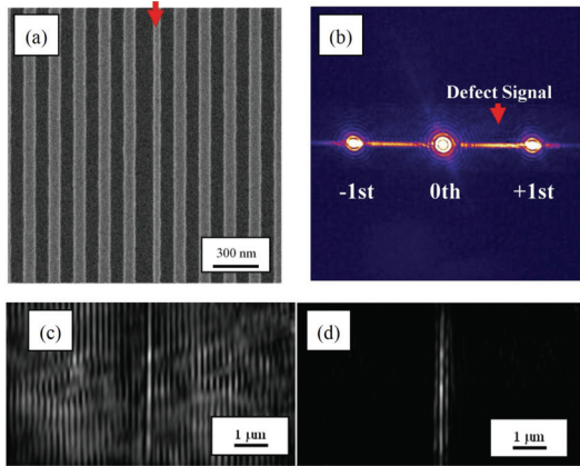
Fig. 8 (a) SEM image and (b) diffraction image of the 30-nm size line defect. (c) Reconstructed image, and (d) that with the periodic signal filtered out.
