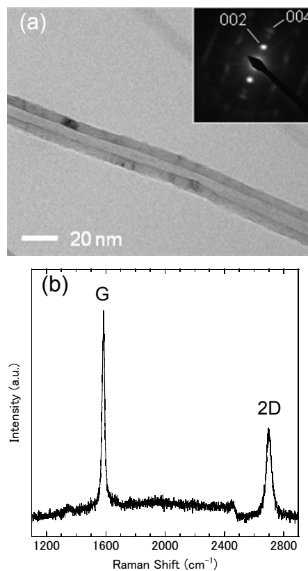
Fig. 1. (a) TEM image of a MWCNT. The inset of (a) shows selected area electron-diffraction pattern. (b) Typical Raman spectrum of multi-layer graphene films.
