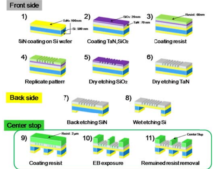
Fig. 3 Fabrication process of the transmission diffraction grating
