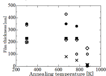
Fig. 3 Dependence on annealing temperature of film thickness obtained from RBS measurement. Circles represent data for FIB-CVD W-DLC1 film fabricated in present work, closed circles represent data for UBMS W-DLC film, closed squares represent data for UBMS DLC film, diamonds represent data for IP DLC film, and crosses represent data for PE-CVD DLC film.
