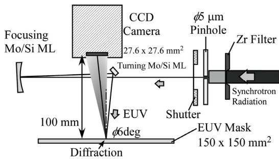
Fig. 2 Schematic view of the CSM system.
