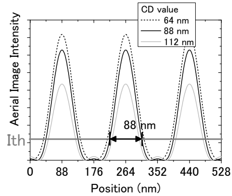
Fig. 4 Calculated intensity profiles of 88 nm L/S patterns, which have varied absorber widths of 64, 88, and 112 nm.
