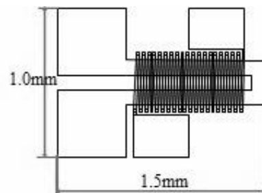
Fig.1 Outline of MI sensor. The number of turns on the coil was 20. The width of the Au wire is 20μm.
