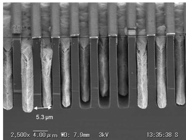
Fig. 4: SEM image of high aspect ratio microstructures.
