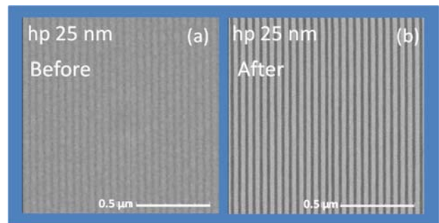
Fig. 7 CD-SEM images of 25-nm-width line and space resist (ZEP520A) pattern (a) before and (b) after the improvement of the grating stage.
