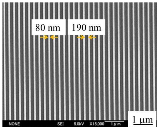
Fig. 3 SEM image of imprinted pattern.
