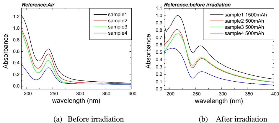
Fig.1 Optical absorbance for (a) before and (b) after UR-irradiated samples (from 1 to 4) of \text{GeO}_2 -doped \text{SiO}_2 film on silica substrate. The UR peak energy is 50eV. Each sample has different amount of original defects which are shown in the spectra in (a). The amount of defects after the irradiation depends on the original ones.
