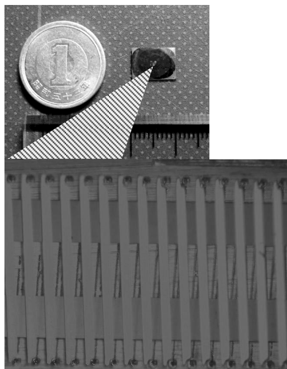
Fig.3 The completed sensor.
