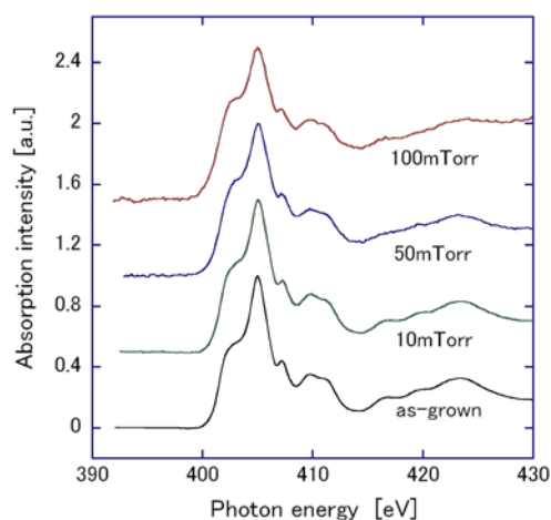
Fig.2 NEXAFS spectra of nitrogen K-edge of n-GaN crystals etched with He plasma obtained by the TEY method.
