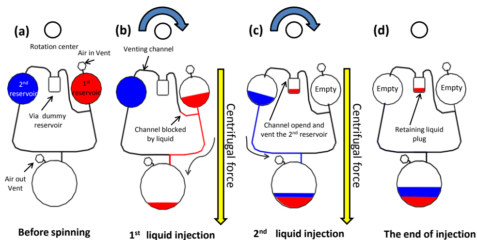
Figure 2: Sequencing method (a) initial state of flow sequencing (b) 1 st liquid injection (vent channel of the 2 nd reservoir is blocked by 1 st liquid) (c) 2 nd liquid injection (following 1 st liquid injection) (d) sequencing completed (both reservoirs are empty)
