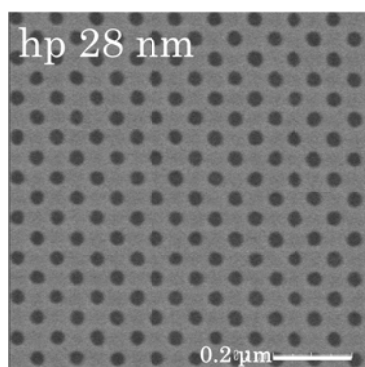
Fig.11 Replicate hole resist pattern (ZEP520A) of hp 28 nm by the four-luminous-flux interference exposure using the four-window diffraction grating.
