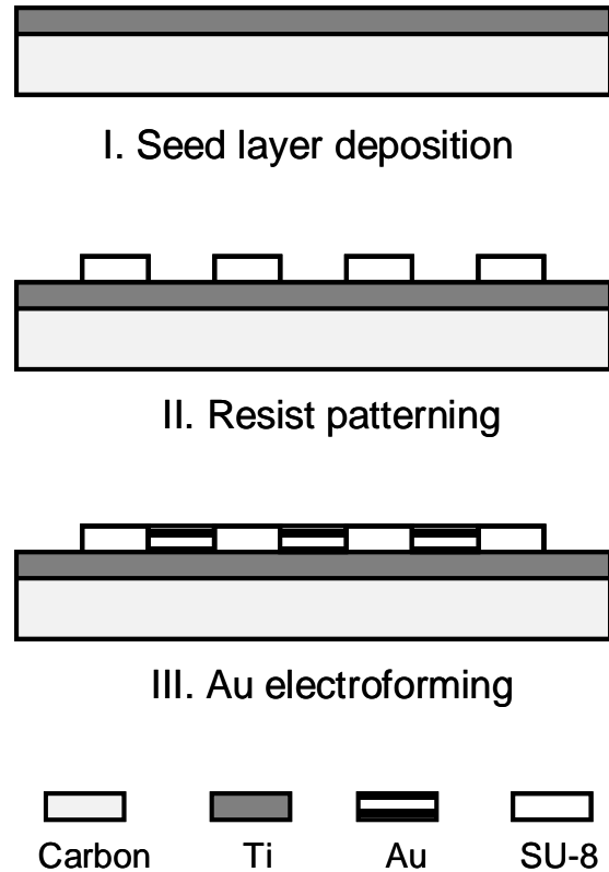
Fig. 1: New fabrication process of X-ray mask.
