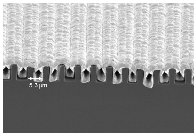
Fig. 2: SEM image of defective Au microstructures.
