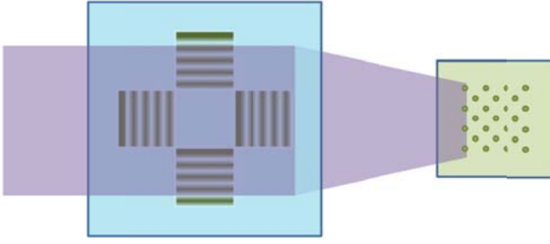
Fig. 8 Hole pattern replication by the four-luminous-flux interference exposure using the four-window diffraction grating.
