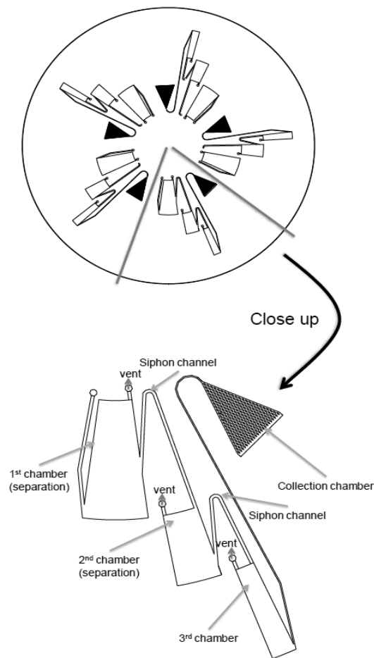
Figure 1 Schematic layout of blood separation
