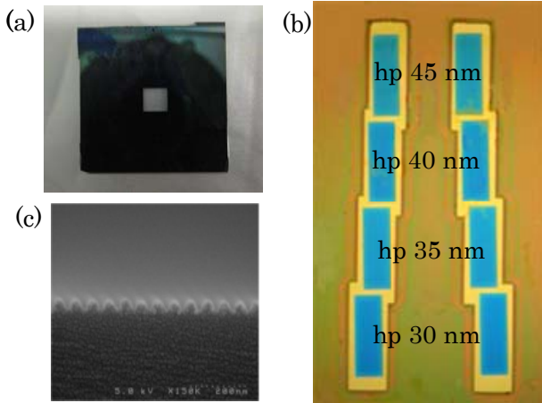
Fig. 4 Fabricated transmission diffraction grating; (a) top view of the transmission grating, (b) arrangement of four sets of the two-windows of diffraction grating, and (c) cross sectional view of the hp 30 nm diffraction gratings before back etching the Si substrate.
