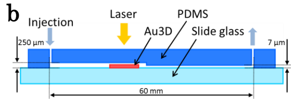
Fig.3: (a) Photo image of microfluidic device. (b) Cross section of microchannel in the microfluidic device (a). Au3D width is 6 mm, height is about 3 \mu\text{m} . Slide glass thickness is 1 mm. PDMS thickness is about 2 mm.
