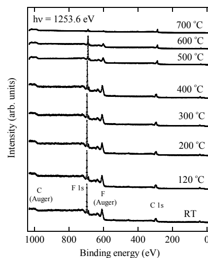
Figure 2. Wide scan of the photoelectron spectra of the F-DLC thin films as a function of the temperature. The photoelectron spectra in this figure were normalized by the C 1s peak intensity.
