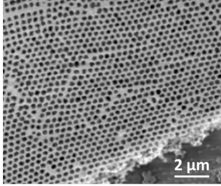
Fig.1: SEM image of Au3D. The diameter of the holes is about 600 nm.
