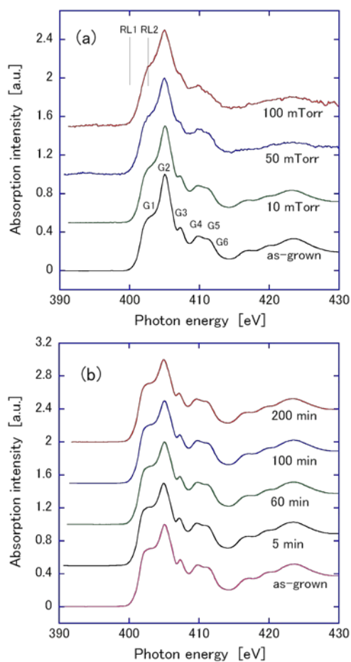
Fig.1 NEXAFS spectra of nitrogen K-edge of n-GaN crystals etched with N 2 plasma obtained by (a):TEY and (b):TFY method at the angle of incidence of 90° from the surface.
