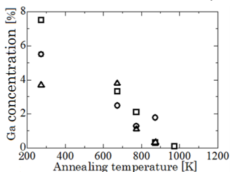
Fig. 1 Dependence on annealing temperature of Ga concentration in W-DLC and DLC films fabricated by FIB-CVD. Circles represent data for FIB-CVD W-DLC1 film fabricated in present work, squares represent data for FIB-CVD W-DLC2 film fabricated in previous work, and triangles represent data for FIB-CVD DLC film fabricated in previous work. Points at 273 K indicate Ga content as-deposited.
