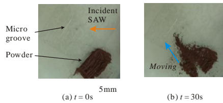
Figure 3. Photographs of powder moved by reflected SAW.
