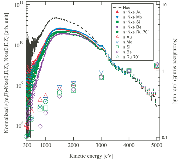
Figure 2 Kinetic energy dependences of the number of xenon ions N_{Xe}(0, E, \bar{Z}) and the sputtering rates s(m, E) .
