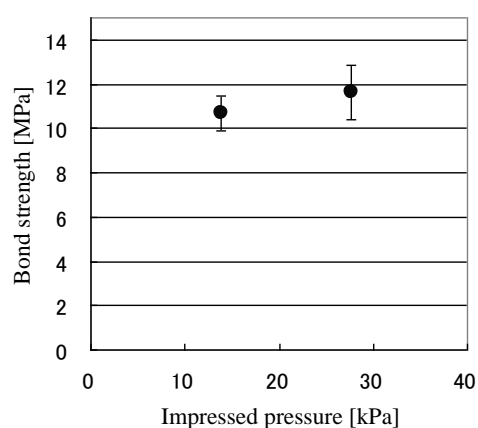
Figure 2. Measurement results of bond strength.
