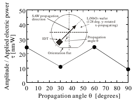
Figure 2. Relationship between SAW propagation angle against orientation flat and SAW amplitude / electric power applied to IDT. Here, \square is 2\square .
