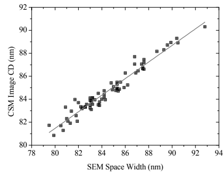
Fig. 9 CD value relationship measured using CSM and by CD-SEM of the EUV mask.
