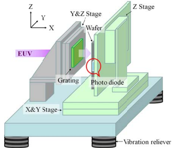
Fig. 5 Stage setup in the EUV-IL exposure tool
