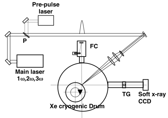
Figure 1. Experimental setup to obtain data of EUV emissions from a cryogenic rotating Xe target. FC represents the Flying Circus III energy generator, and TG is a transmission grating.
