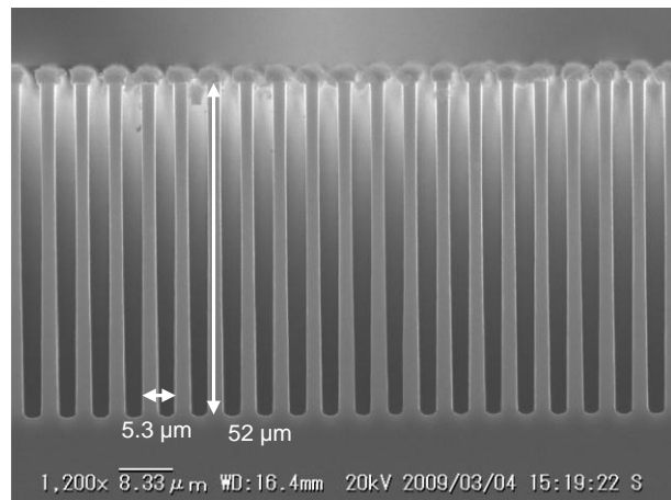
Fig. 1: SEM image of Si microstructures using ICP-RIE.
