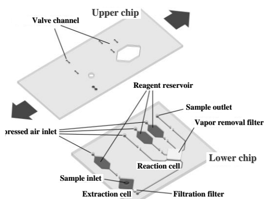
Figure 1. Schematic diagram of amino acid derivatization device.
