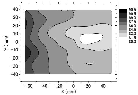
Fig. 8 Results of evaluation of image CD uniformity for CSM. The number of sampling points is 10 \times 9 , where the 88 nm L/S patterns fabricated by the same process are located with 13 mm steps.
