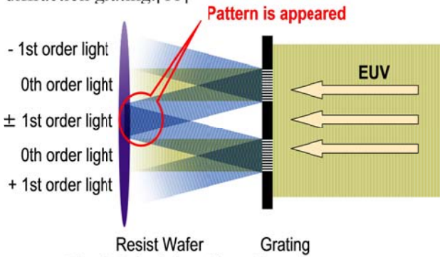
Fig. 2 Principle of interference exposure
