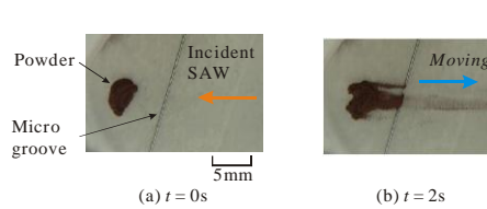
Figure 4. Photographs of powder moved by transmitted SAW.
