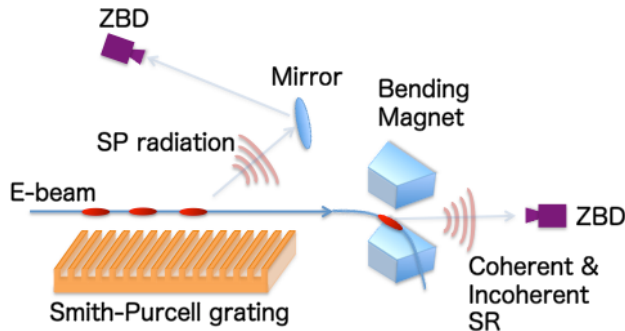
Fig.2 The generation and measurement of Terahertz radiations at LEENA; The synchrotron radiation from the bending magnet and the Smith-Purcell radiation.
