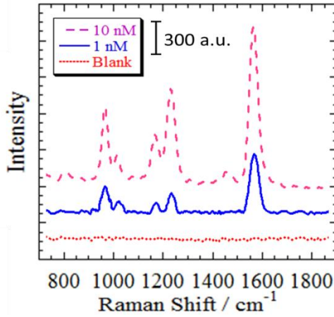
Fig.4: SERS spectra of 4bpy with different concentration (10 nM, 1 nM, Blank) by flow measurement.
