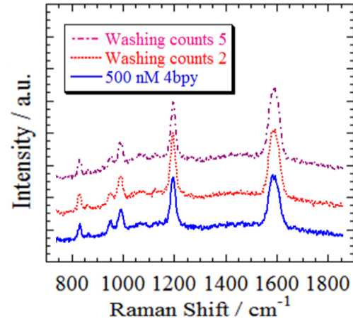
Fig.5: Evaluation of adsorption effect by washing Au3D. Au3D was repeatedly soaked in ultrapure water for 5 min after SERS measurement of 500 nM 4bpy.
