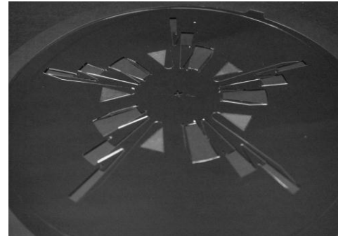
Figure 2 Photo of the fabricated chip The microchannels are fabricated by patterning photoresist SU-8 by x-ray lithography. The fabricated SU-8 chip is locally hydrophilized by exposure UV.
