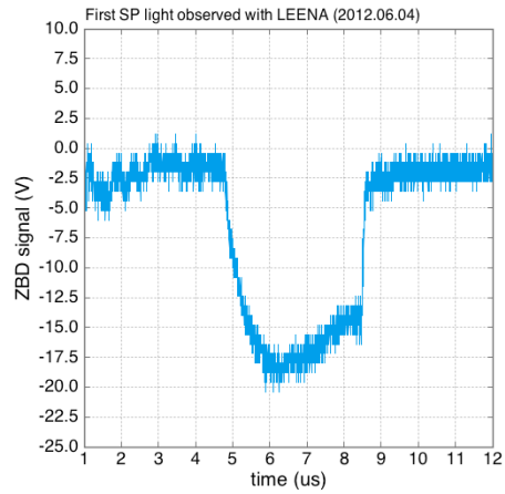
Fig.3 Waveform of Smith-Purcell radiation measured by a Zero Bias Diode.
