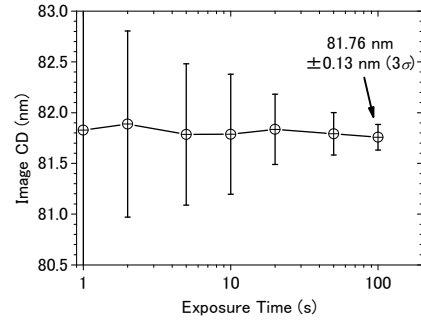
Fig. 7 Repeatability of CSM at various exposure times from 1 to 100 s. The error bar means the three-sigma deviation from the average.
