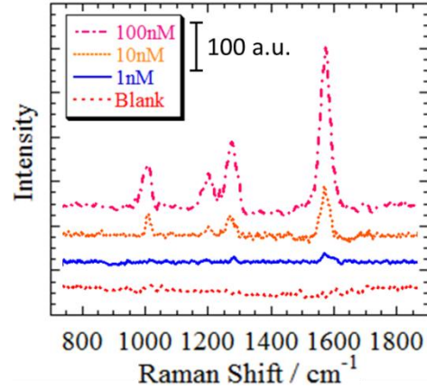
Fig.2: Characteristic enhanced Raman spectra of 4bpy with different concentration (100 nM, 10 nM, 1 nM, Blank) by batch measurement.
