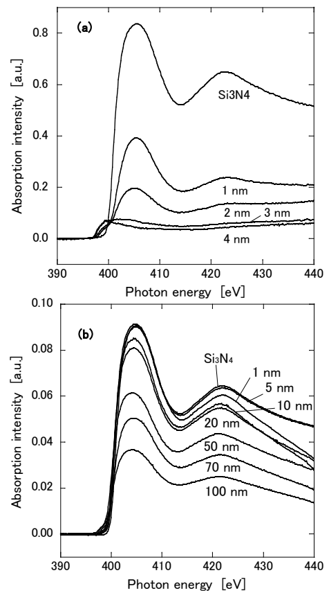
Fig. 2 N-K absorption spectra of \text{Si}_3\text{N}_4 crystal covered with Cr thin film of various thicknesses measured using the (a): TEY and (b): TFY methods.
