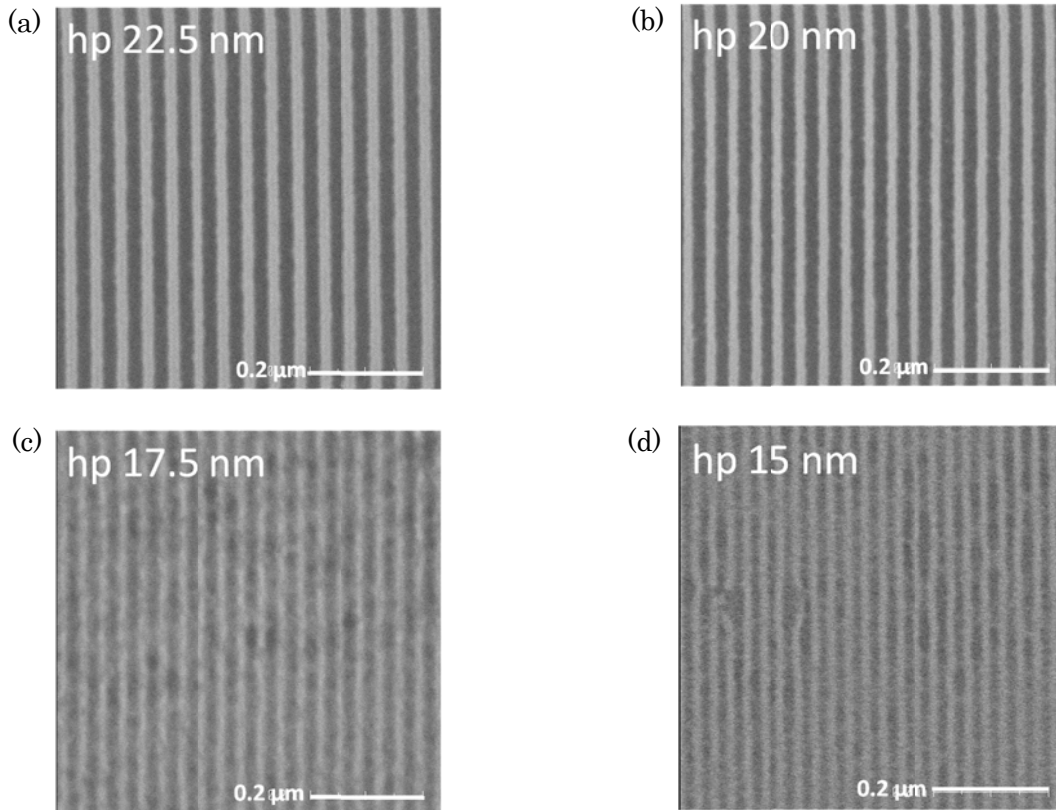
Fig. 10 CD-SEM images of the replicated resist images of the non-chemically amplified negative-tone resist (Inpria); (a) hp 22.5 nm, (b) hp 20 nm, (c) hp 17.5 nm, and (d) hp 15 nm.
