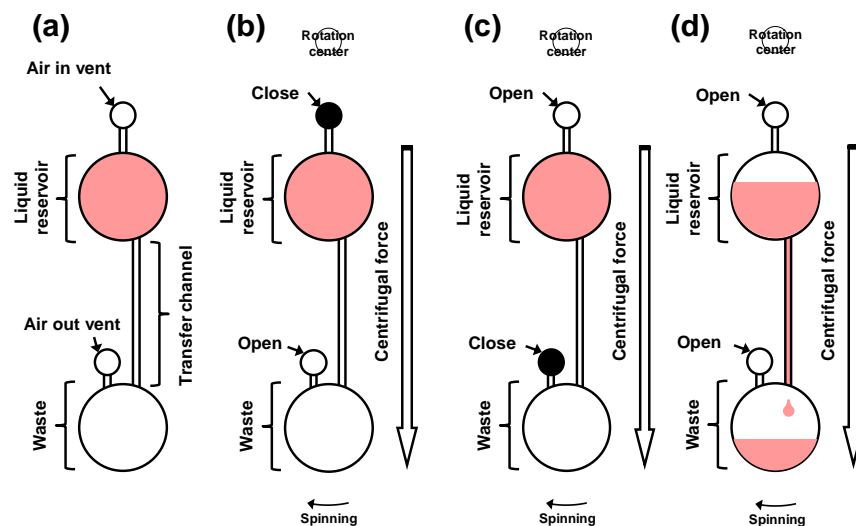
Figure 1: Principle of valving. (a) Initial state of the liquid (liquid is loaded in the liquid reservoir) (b) liquid injection with closed air in vent (liquid does not flow due to lack of air supply from air in vent) (c) with closed air out vent (liquid does not flow due to blocking of air exit) (d) with opened vents (liquid flows and get transported to waste reservoir)
