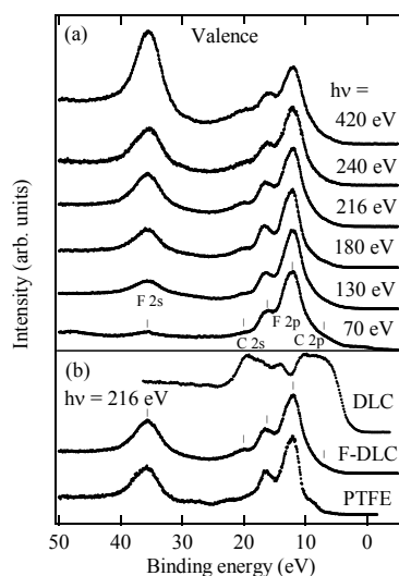
Figure 1. (a) Photoelectron spectra of the valence band region in F-DLC thin films as a function of the photon energy. (b) Photoelectron spectrum of the valence band region in F-DLC thin film was compared with that of the DLC thin film and of PTFE.
