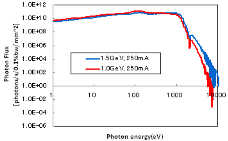
Fig. 1 Photon flux in the BL06
