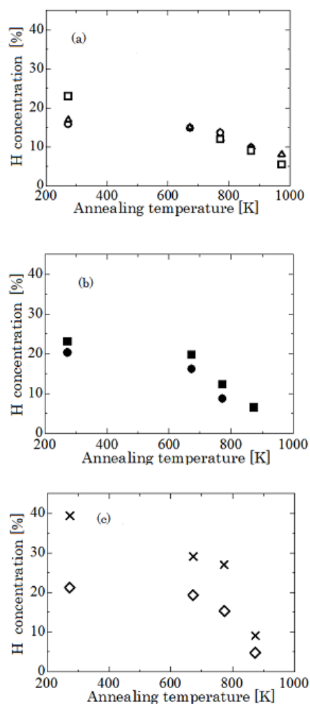
Fig. 2 Dependence on annealing temperature of H concentration: a) Circles represent data for FIB-CVD W-DLC1 film fabricated in present work, squares represent data for FIB-CVD W-DLC2 film fabricated in previous work, and triangles represent data for FIB-CVD DLC film fabricated in previous work; b) Closed circles represent data for UBMS W-DLC film and Closed squares represent data for UBMS DLC film; c) Diamonds represent data for IP DLC film and crosses represent data for PE-CVD DLC film.
