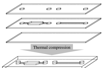
Figure 3. Overview of thermal compression bonding.
