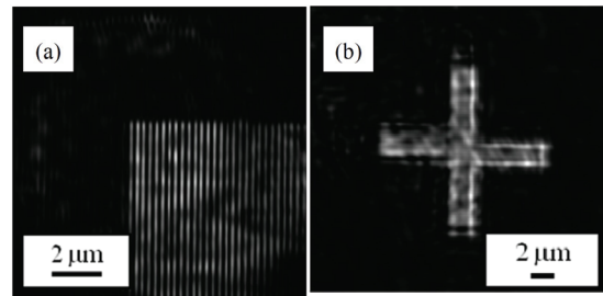
Fig. 6 Reconstructed images of absorber patterns using the CSM. (a) 128-nm L/S pattern. (b) 2- \mu\text{m} width crossed lines.
