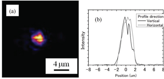
Fig. 5(a) The reconstructed image, and (b) the horizontal and vertical profile of the probe.
