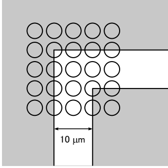
Fig. 4 The schematic of the elbow pattern to reconstruct the illumination probe. The circles indicate the illumination positions.
